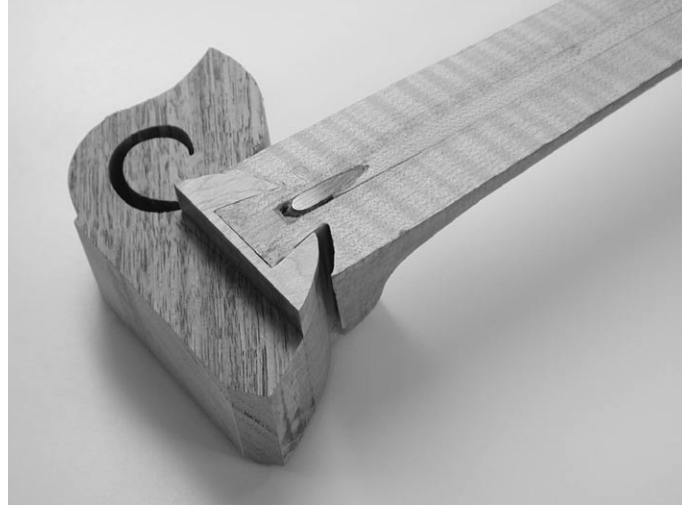
Fig. 8.21 If you prepare the dovetail before attaching the headblock to the rim, be sure to cut the headblock's shape before cutting the cap. If they are cut when glued together, there will be a notch on the treble side of the cap (above) where it appears that the rim will fit, but this is wrong. The cap must overlay the rim as shown in Fig. 8.22 (below).
