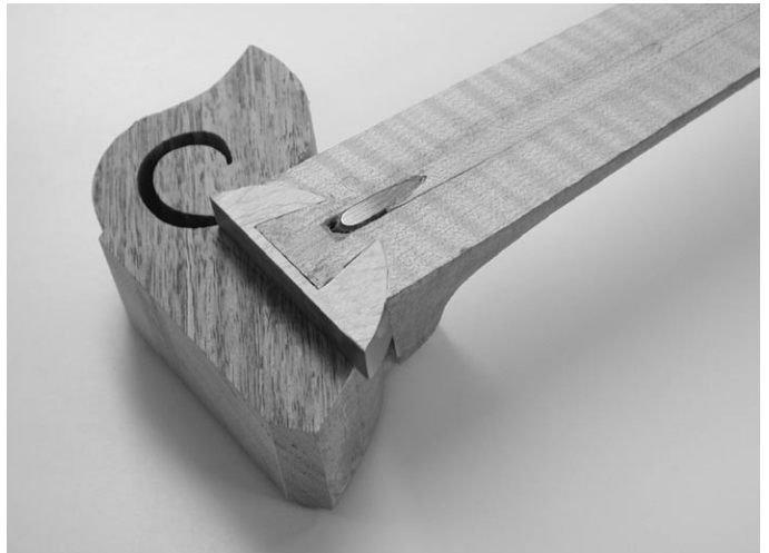
Fig. 8.22 A successful dovetail is an exciting component of an instrument that no one but you will ever see! Compare this photo with Fig. 8.21 and notice how this headblock cap correctly overhangs the headblock on the treble side.
